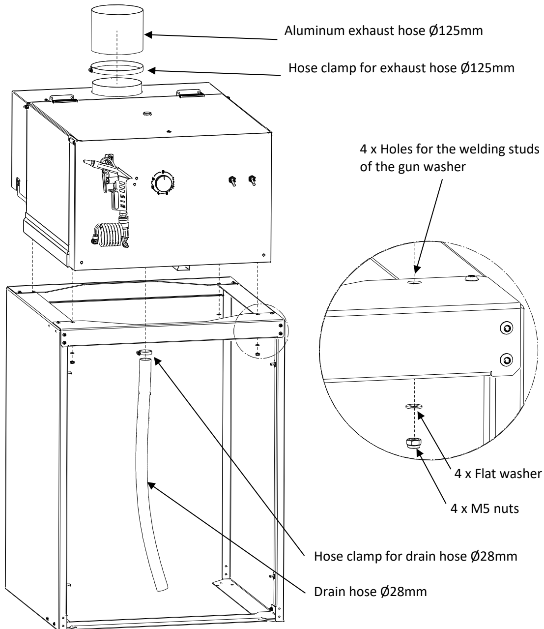
Figure 8-2: Screw starter to base + attach exhaust and drain hose
