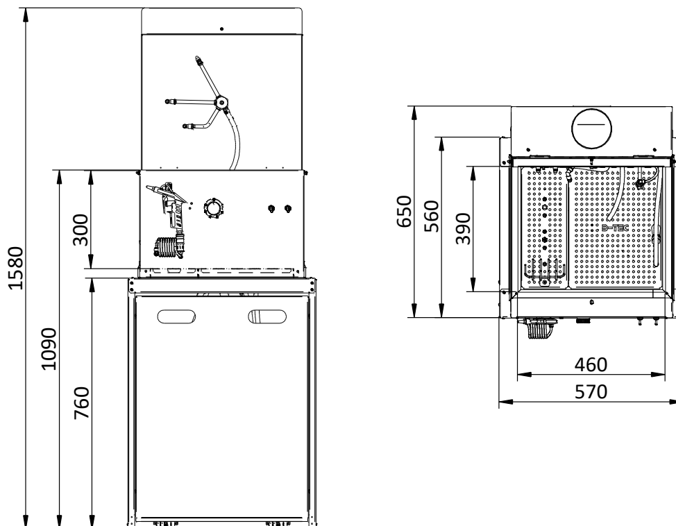
Figure 4-2 – Example Starter-01
