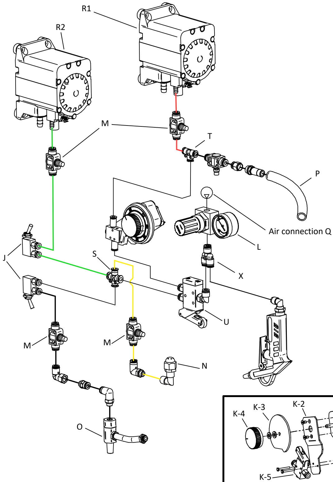
Figure 4-3 – Example Starter-01
