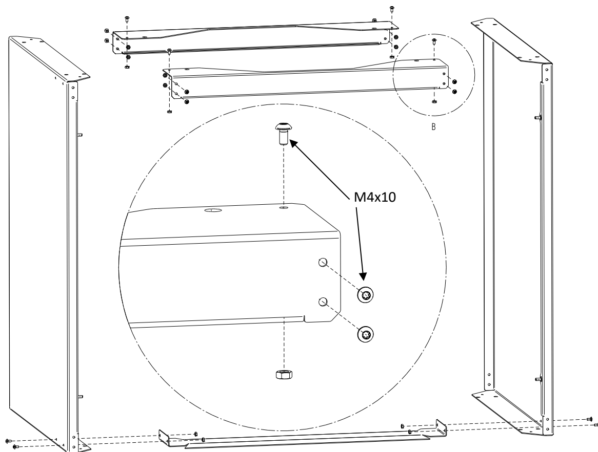
Figure 8-1: Mounting the base
